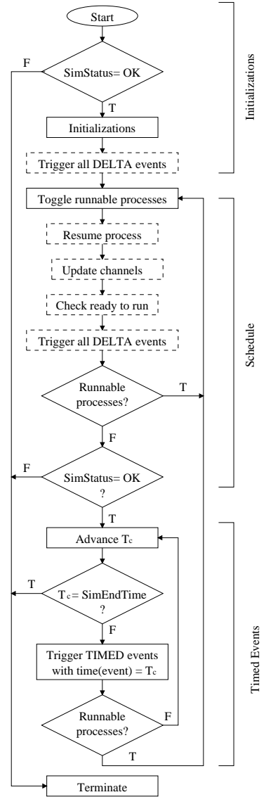
Figure 2: The SystemC simulator
