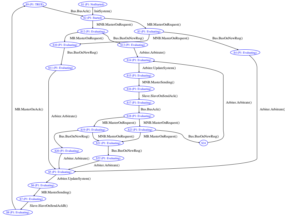
Figure 6: Generated state machine for the bus structure.
