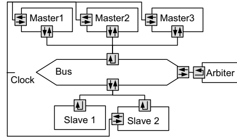
Figure 4: Simple bus structure.
