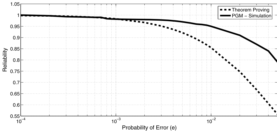
Fig. 4. Reliability for majority gate based full adder.
