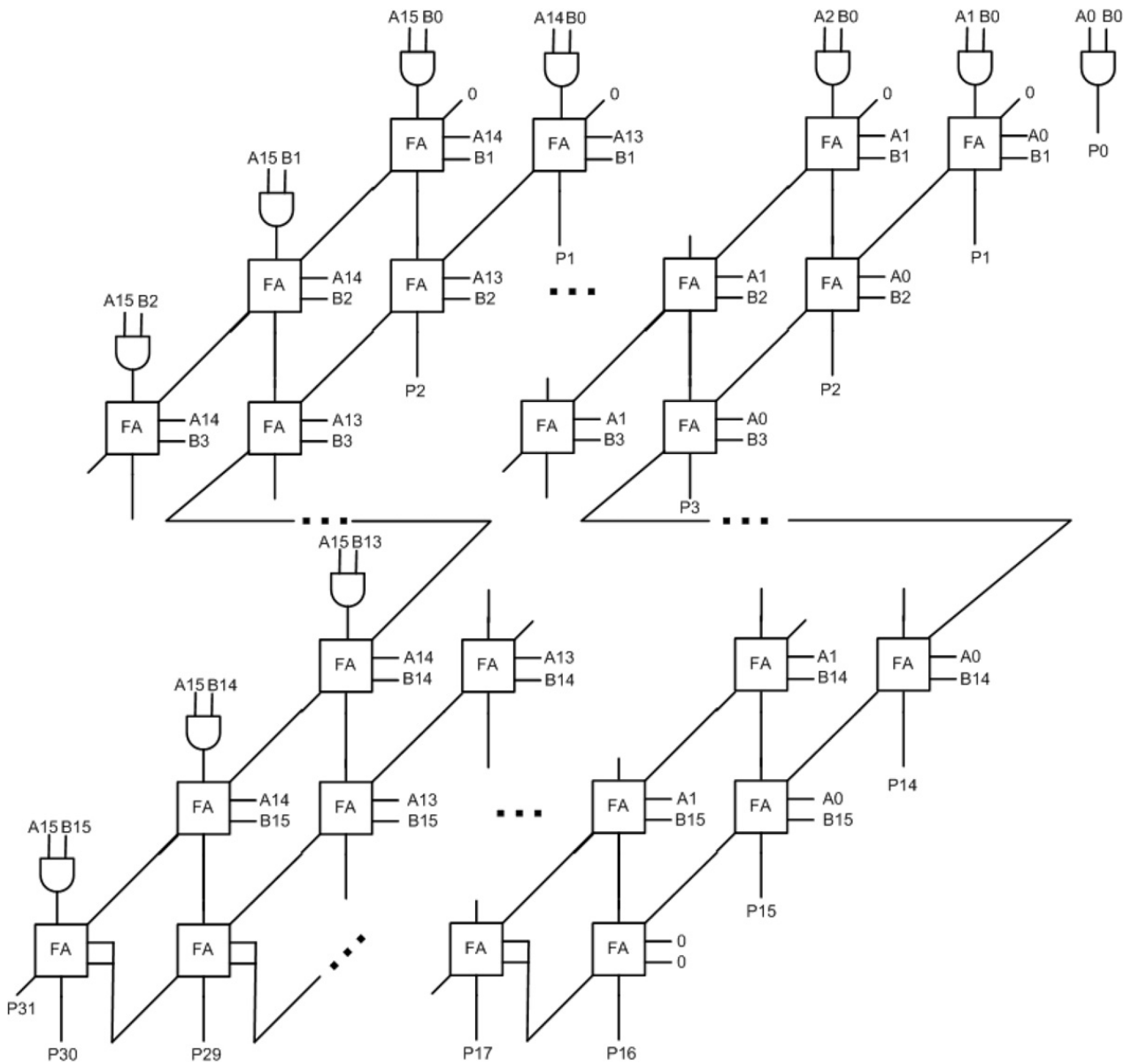
Fig. 5. ISCAS-85-C6288 benchmark.
