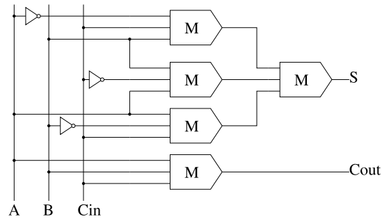
Fig. 3. Majority gate based full adder.
