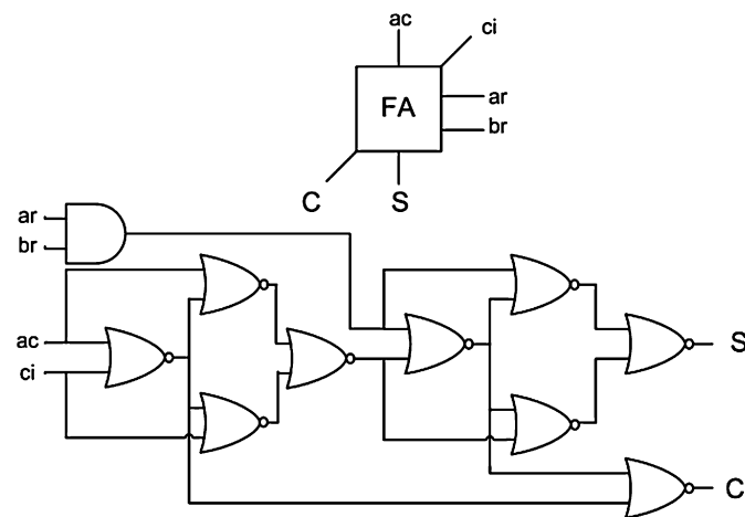
Fig. 6. ISCAS-85-C6288 full adder cell.
