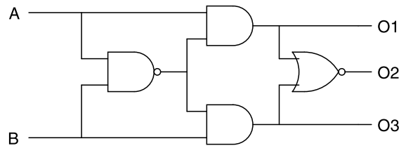
Fig. 2. A 2-bit comparator.
