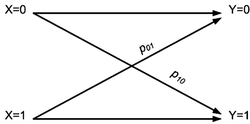
Fig. 1. Binary asymmetric channel with crossover probabilities.
