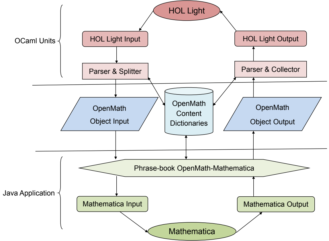
Figure 3.1: Flow of Connecting HOL Light to Mathematica
