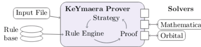
Figure 1.1: Architecture of the KeYmaera Prover [55]
